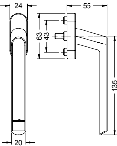
Fenstergriff Standard Standard window handle
