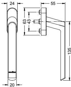
Fenstergriff Standard Standard window handle
