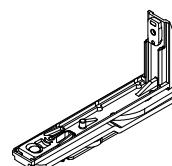
Ecklager Corner pivot 1.2 – 130 kg 1.6 – 160 kg
